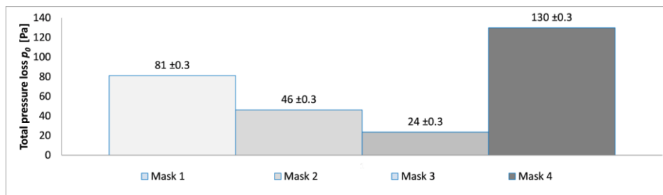
Fig. 4. Comparison of the average total pressure drop for the materials of masks 1–4, for flow rates from 300 to 2000 l/h
