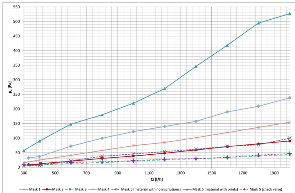
Fig. 6. Total pressure drop curves for masks 1–5, for flow rates from 300 to 2000 l/h
